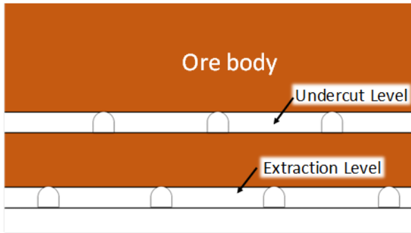
③ Undercutting
