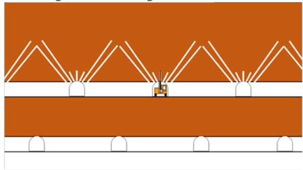
④ Drilling for drawbell
